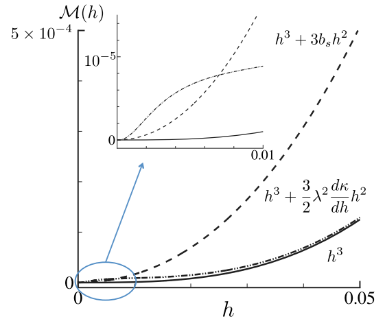
FIG. 2 (color online). Comparison of the mobility with and without slip [ \mathcal{M}(h) = h^3 —, \mathcal{M}(h) = h^3 + 3b_s h^2 , b_s = 10d_0 ----, \mathcal{M}(h) = h^3 + (3/2)\lambda^2(d\kappa/dh)h^2 , \lambda = 10d_0 , \theta_Y = \pi/12 —·—]. While Navier slip is global, our proposed slip model is localized to the contact-line region, where it dominates the Navier slip, consistent with molecular simulations [28,29].
