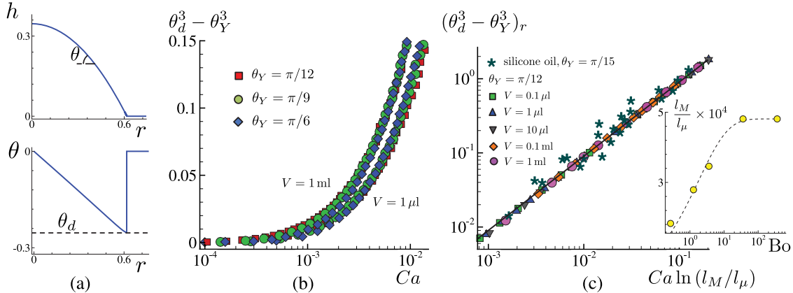
FIG. 4 (color online). (a) The dynamic contact angle is defined at the inflection point of the drop profile (top panel), where its slope (bottom panel) reaches a plateau [ \tan \theta = (h_*/R_f)(dh/dr) ]. (b) The dynamic contact angle, \theta_d , follows the Cox-Voinov law \theta_d^3 - \theta_Y^3 = 9Ca \ln(l_M/l_\mu) , but increases with the volume of the liquid. (c) The nonlocal influence of bulk flow can be conflated into the macroscopic length scale, l_M , leading to a collapse of the dynamic contact angle data for the different volumes onto a single curve (the solid line represents the Cox-Voinov law). The stars represent the classic experiments of Ref. [43] corresponding to the silicone oil-air interface in a capillary tube ( l_M/l_\mu \approx 1.25 \times 10^3 ). The rescaled contact angle data from the model accounts for the fact that the microscopic length scale l_\mu is magnified by 10^4 in the simulations: (\theta_d^3 - \theta_Y^3)_r = \theta_d^3 - \theta_Y^3 + (9 \ln 10^4)Ca . (Inset) An approximate fit l_M/l_\mu = 4.8 \times 10^4 \times [1 - \exp(-0.75Bo^{1/2})] is shown as the dashed line.
