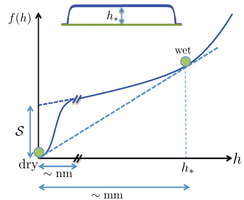
FIG. 1 (color online). Schematic of the tangent construction on the bulk free energy, f(h) , leading to the coexistence of wet, h = h_* , and dry, h = 0 , states. In the absence of intermolecular forces, the bulk free energy does not reduce to the solid-gas interfacial energy as h \rightarrow 0 unless \mathcal{S} = 0 , which implies complete wetting [10].
