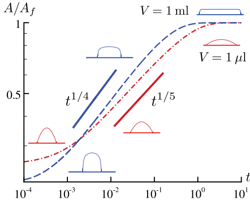
FIG. 3 (color online). The rate of spreading is influenced by the volume of liquid. For small volumes ( Bo \lesssim 1 , ---), capillary forces are dominant and the drop takes the shape of a spherical cap while viscosity resists the spreading, leading to Tanner's law A \sim t^{1/5} . For large volumes ( Bo \approx 360 , ---), gravity dominates, leading to a t^{1/4} scaling; the liquid puddle takes the shape of a pancake at equilibrium. A_f is the final equilibrium area and \theta_Y = \pi/12 .
